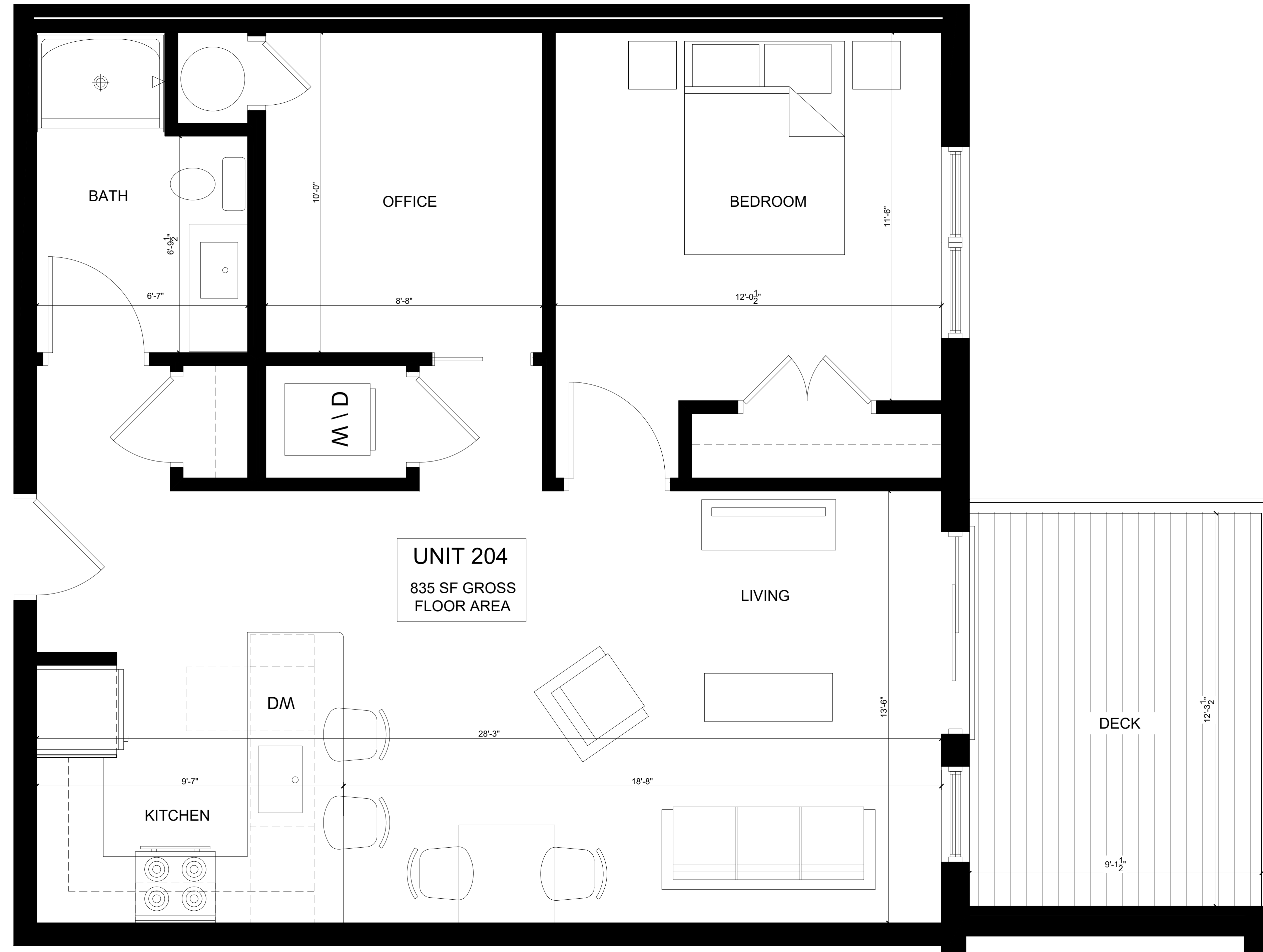
1 UNIT 204 PLAN (UNITS 304, 404, 504 SIMILAR) 1/2" = 1'-0"
