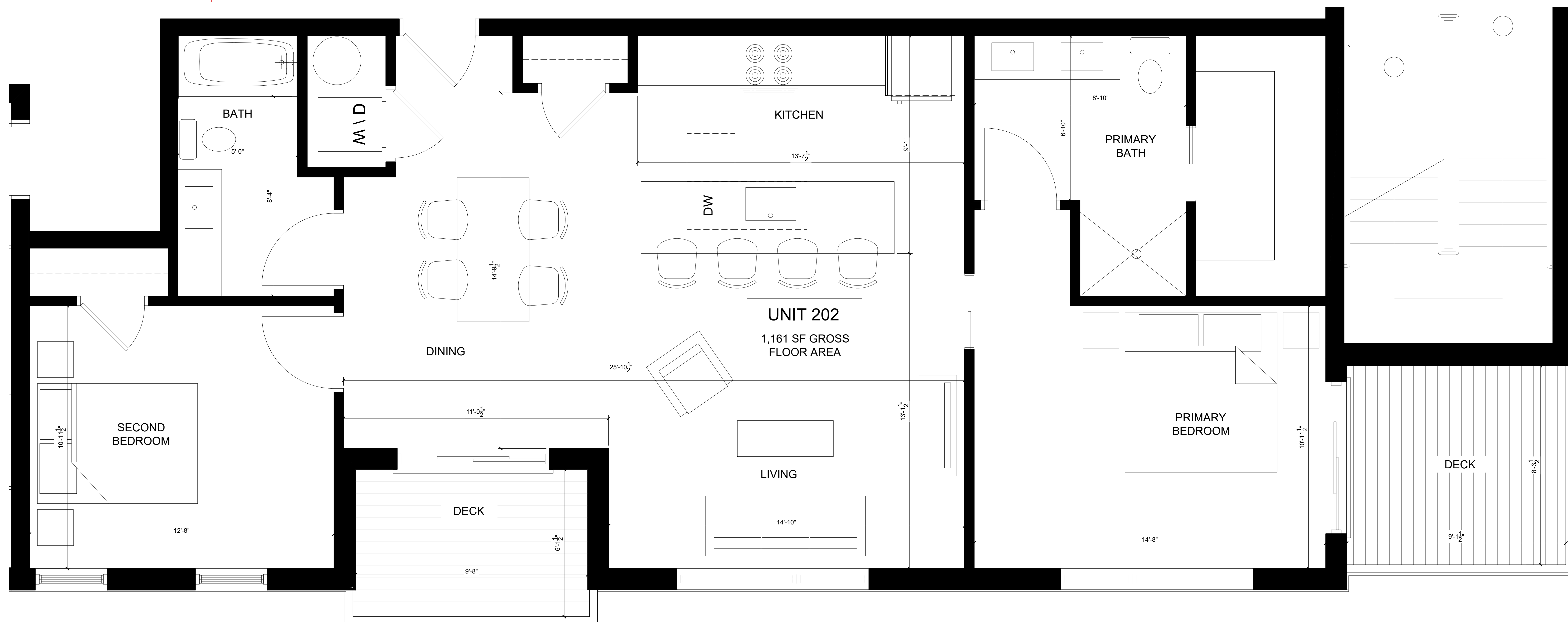
1 UNIT 202 PLAN (UNITS 302, 402, 502 SIMILAR) 1/2" = 1'-0"
