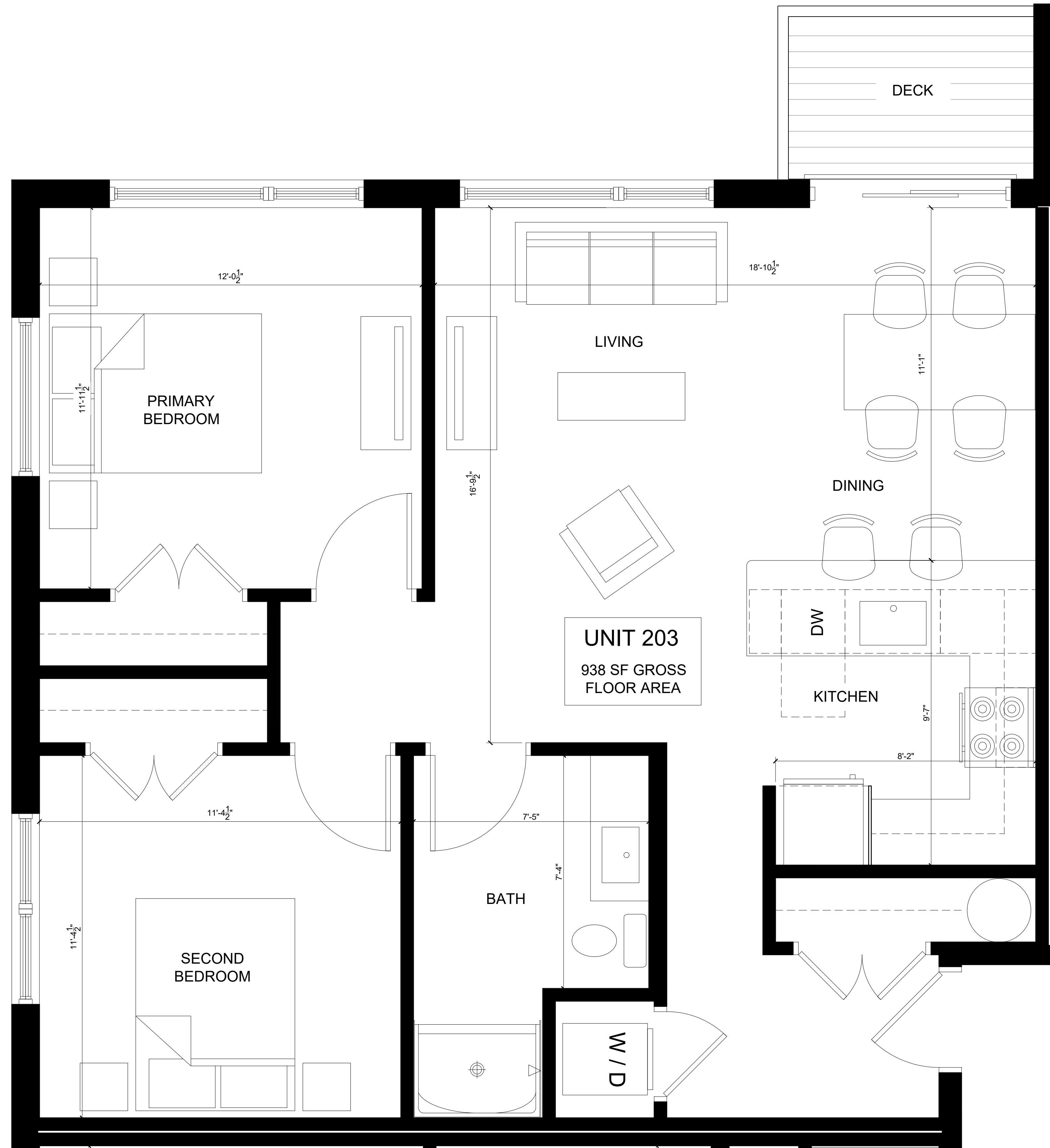
1 UNIT 203 PLAN (UNITS 303, 403, 503 SIMILAR) 1/2" = 1'-0"
